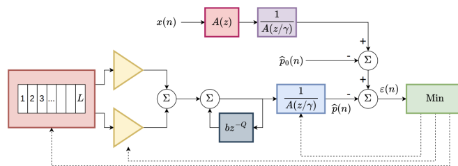
CELP Architecture
