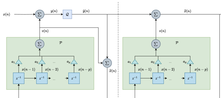
Block Scheme
